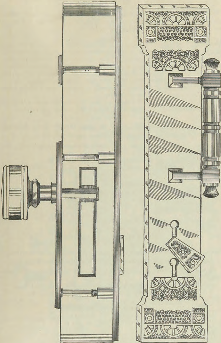
Sectional view.
