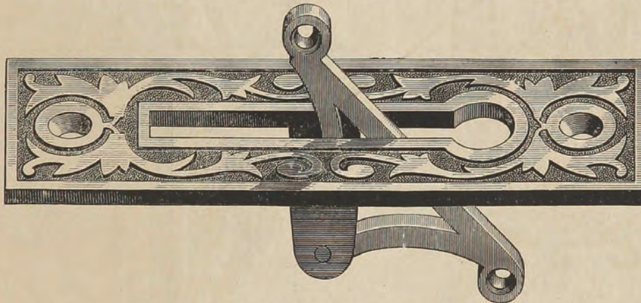
MORTISE BELL CRANK No. 752.
